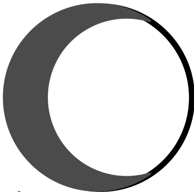
Waxing Gibbous
