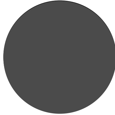
New Moon
