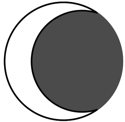
Waning Crescent
