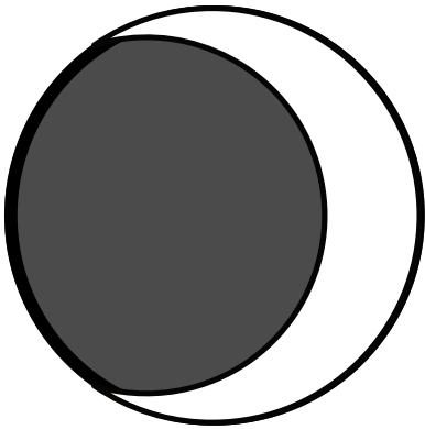
Waxing Crescent
