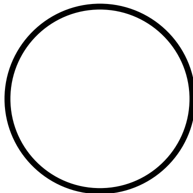
Full Moon
