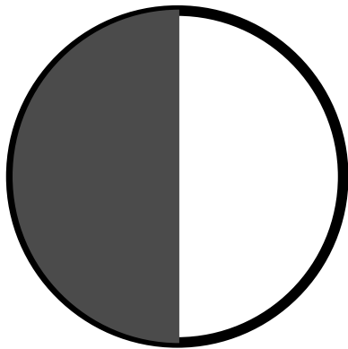
First Quarter
