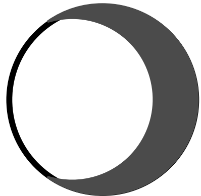
Waning Gibbous
